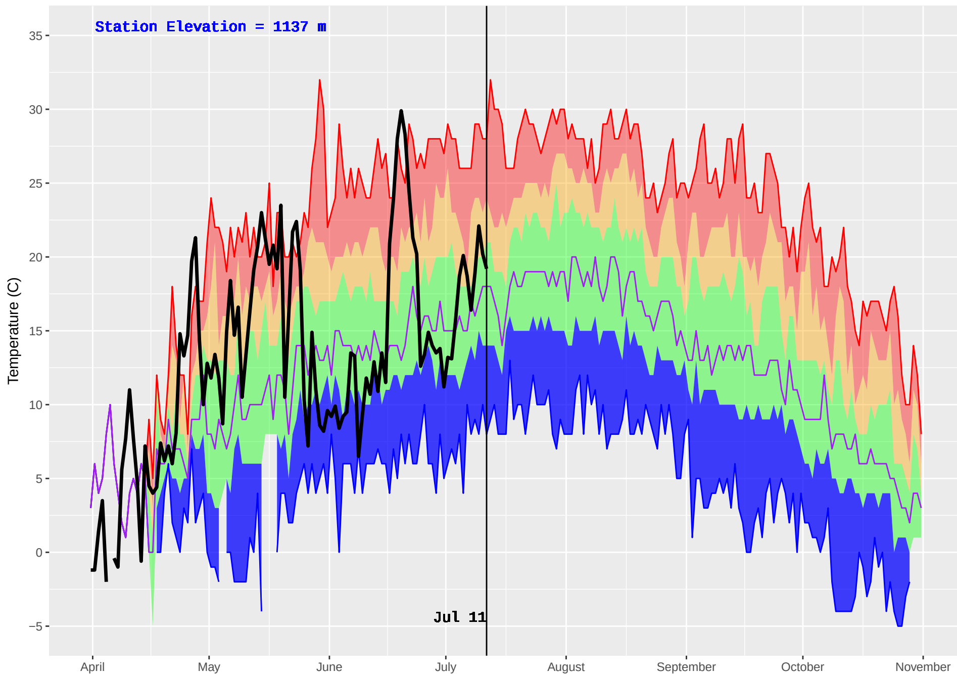
KLUSKUS (166) : Historical (1982–2016) and Current (2018) Noon Temperature
